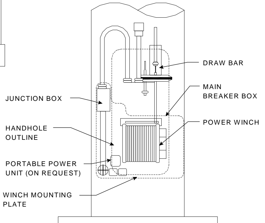
SECTION DETAIL
