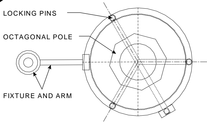
POLE TOP VIEW
